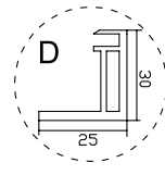
Frame cross-section
