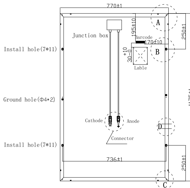
Install hole (7*11)
