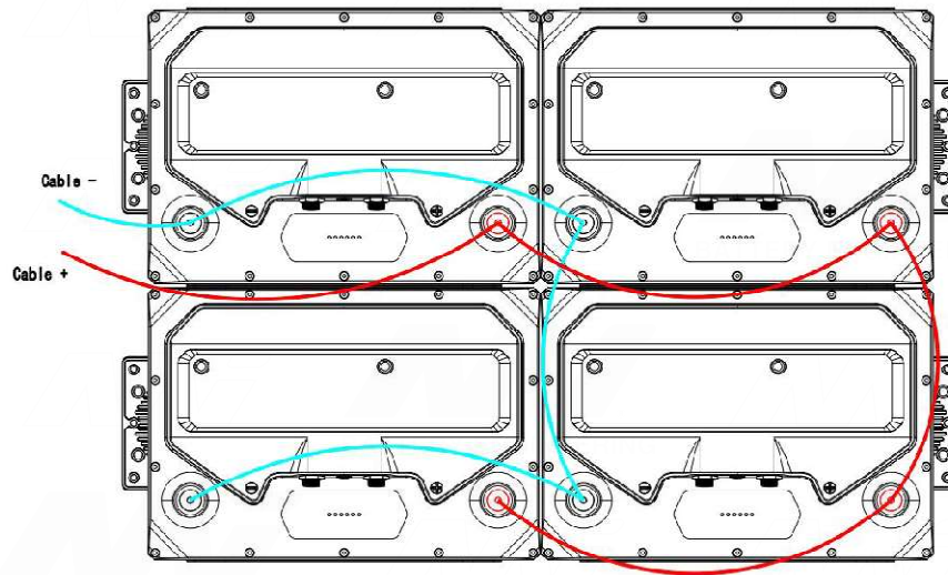
Figure 5-4: VRLV2560, 5120 Batteries Power Cable Connection Diagram
